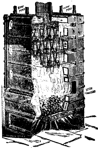
"PERFECT" HOT WATER HEATER.
